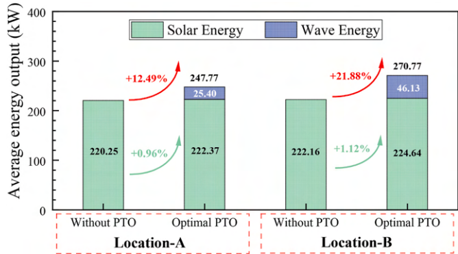
Fig. 21. The power generation of the hybrid system under selected operational sites.
