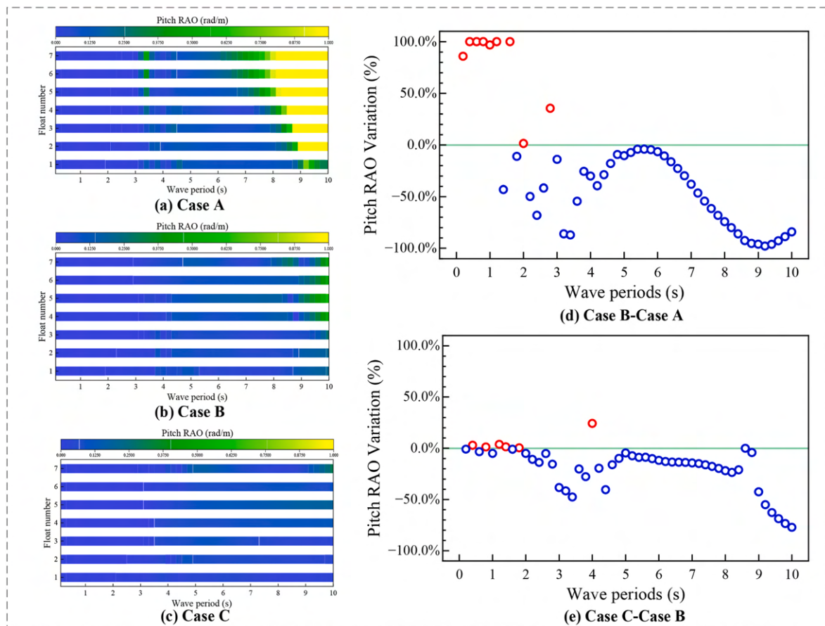
Fig. 7. Comparison of pitch RAOs for three FPV array configurations.
