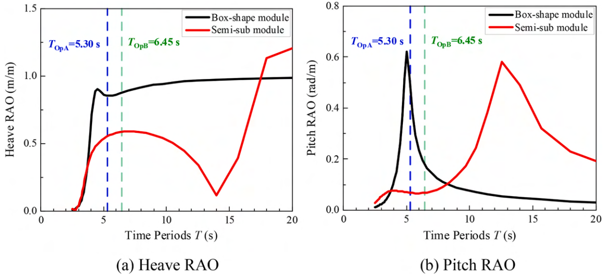
Fig. 2. Motion response RAOs between Box-type and Semi-submersible floating modules.
