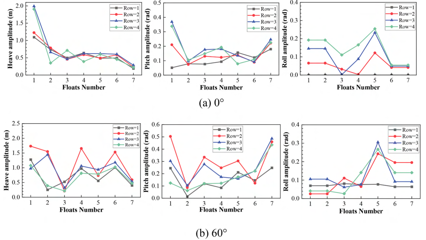
Fig. 15. Motion response FPV array with varying numbers of rows ( T = 5.30 \text{ s} ).
