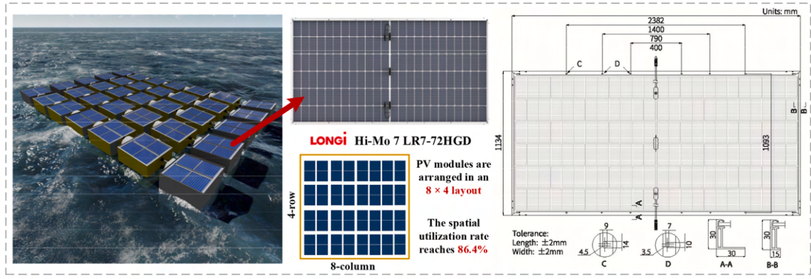
Fig. 4. Schematic diagram and main dimensions of the photovoltaic module.
