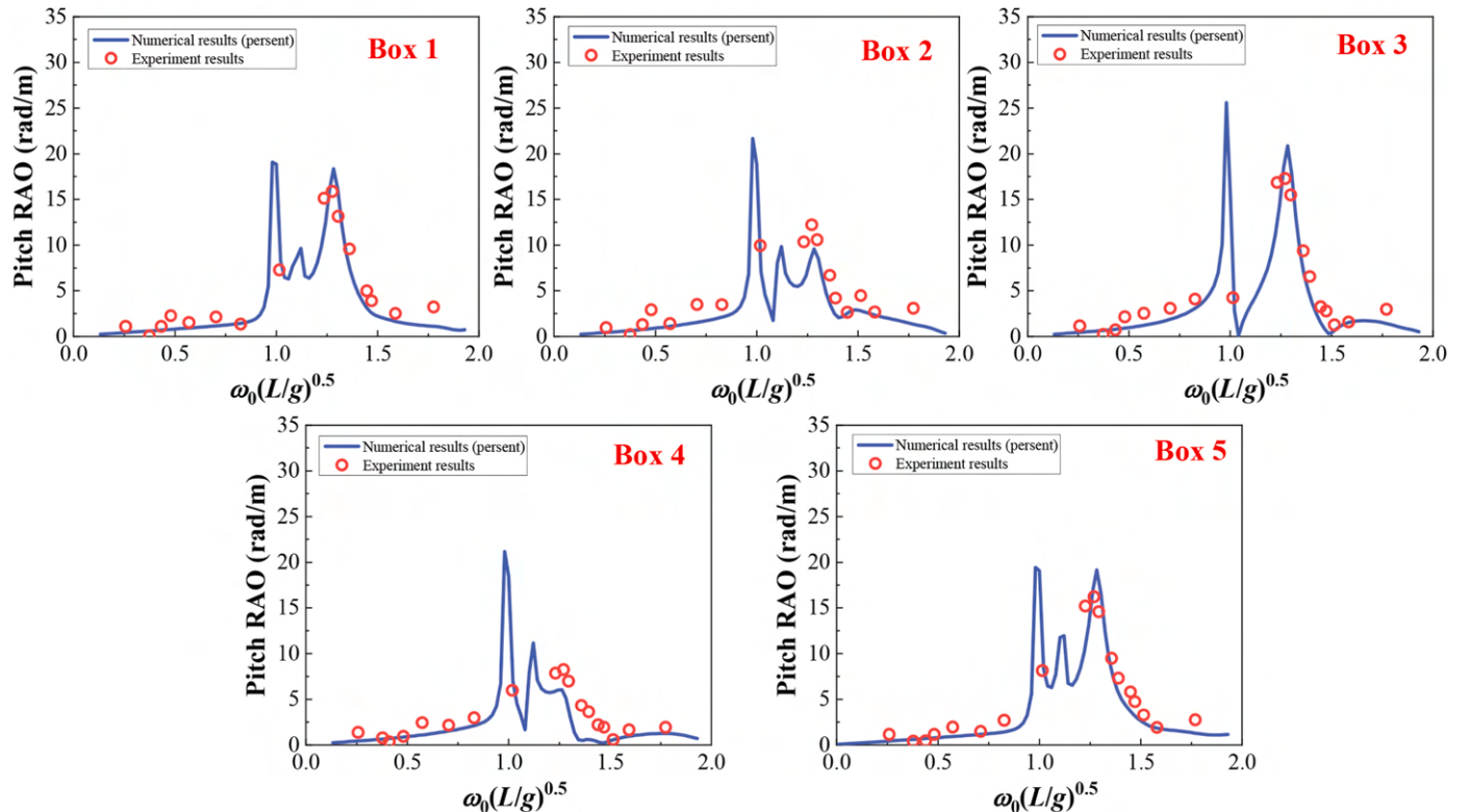
Fig. 6. Comparison of the pitch RAO of the boxes between the proposed numerical model and experimental results.
