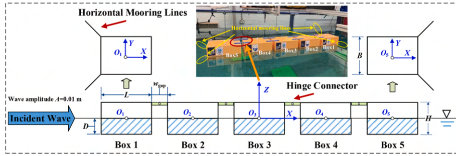
Fig. 5. Schematic of the validation model of a 5-box system with hinge assembly.
