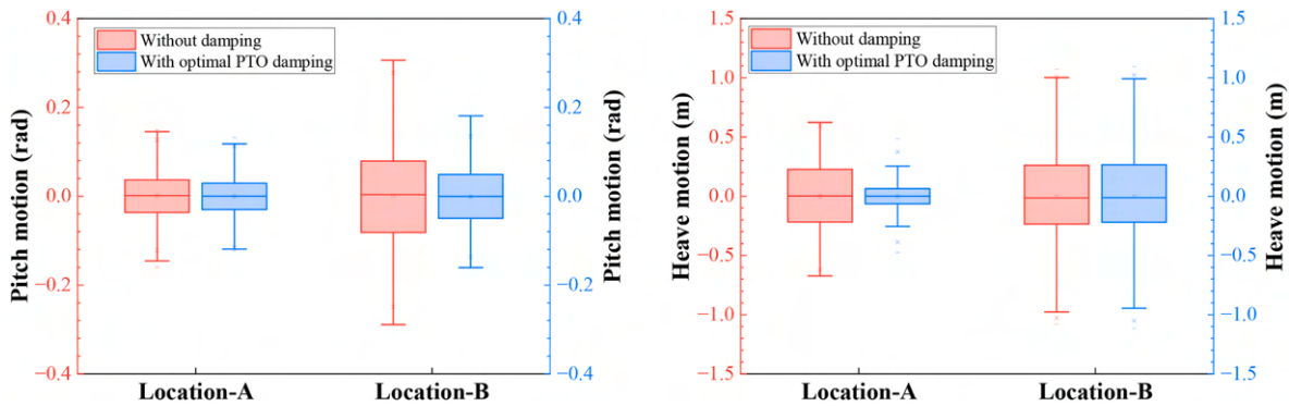
Fig. 20. Box-plot of the motion responses of the float with maximum motion.
