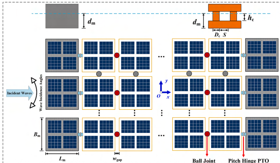
Fig. 3. Sketch and configuration of the dual-module FPV array system.
