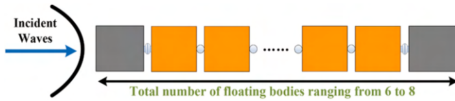
Fig. 10. Top view sketch of a row of FPV array.
