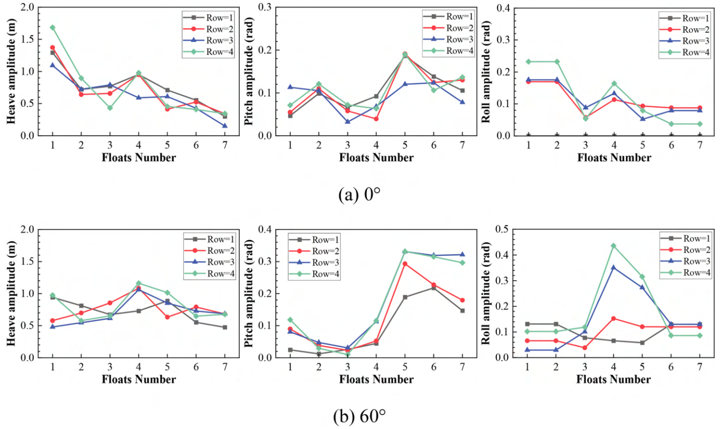
Fig. 16. Motion response FPV array with varying numbers of rows ( T = 6.45 s).
