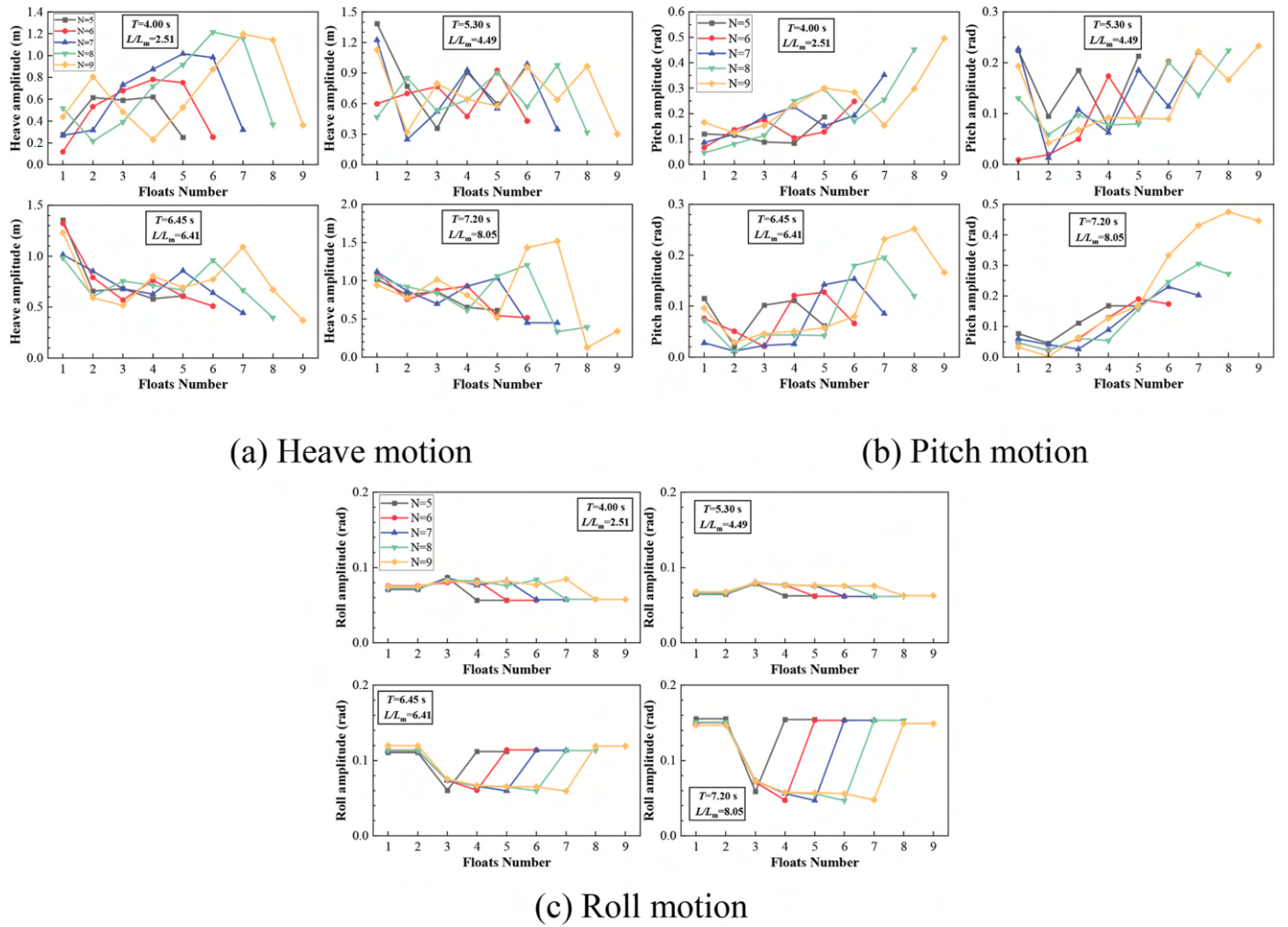
Fig. 13. Motion responses of a single-row array with varying numbers of floats at four representative wave periods ( 60^\circ wave incidence).
