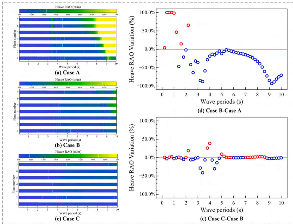
Fig. 8. Comparison of heave RAOs for three FPV array configurations.
