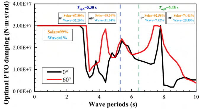
Fig. 17. Optimal PTO damping under different wave conditions.
