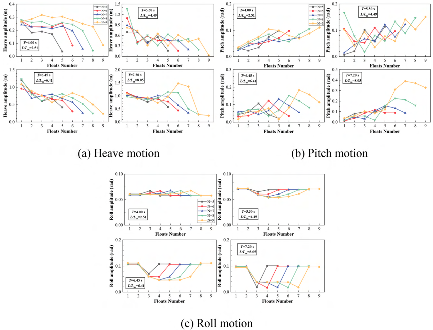
Fig. 12. Motion responses of a single-row array with varying numbers of floats at four representative wave periods (30° wave incidence).
