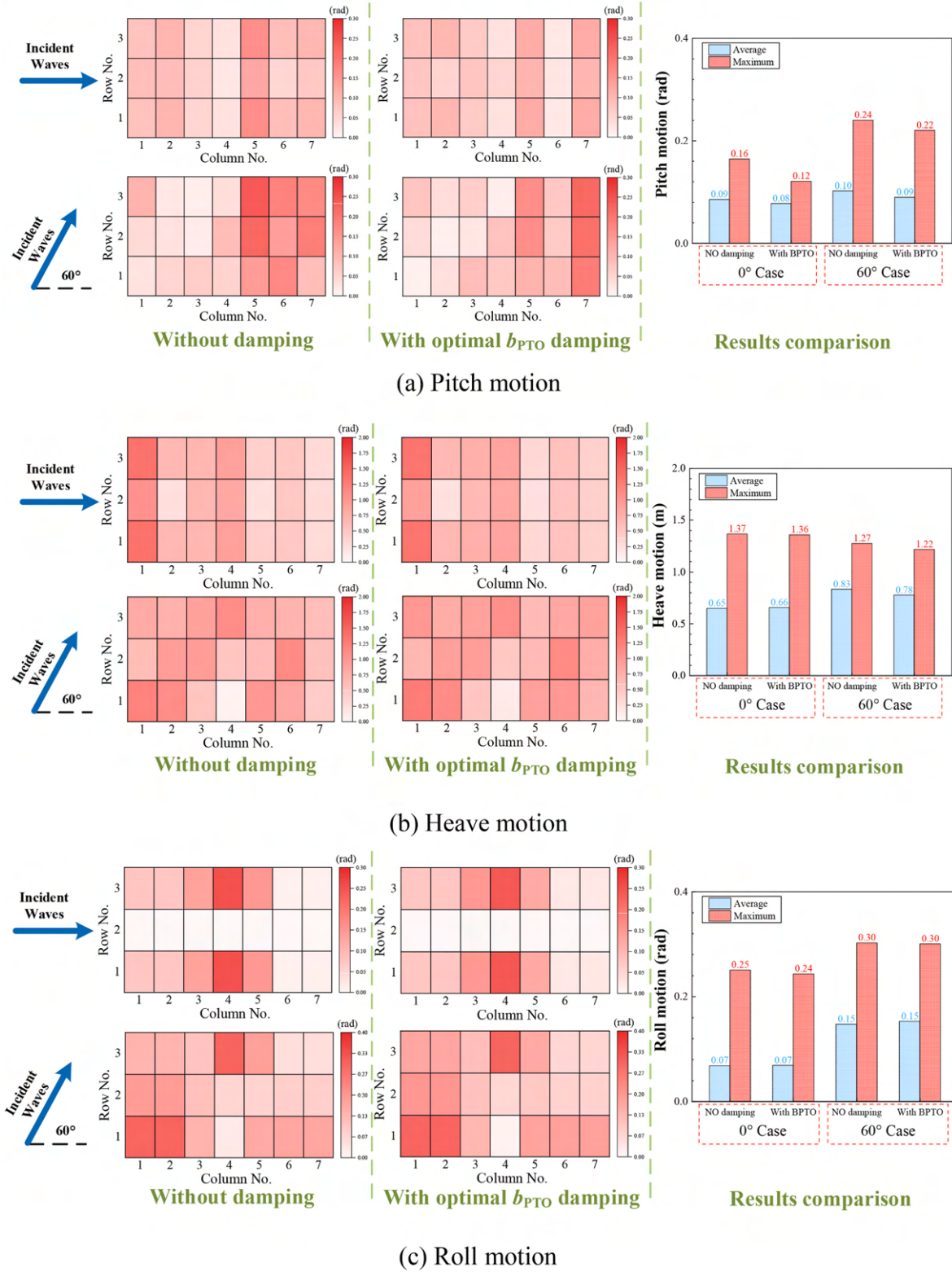
Fig. 19. Impact of optimal b_{PTO} damping on the motion response of the array at T = 6.45 s.
