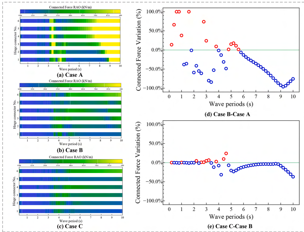
Fig. 9. Comparison of connector force RAOs for three FPV array configurations.
