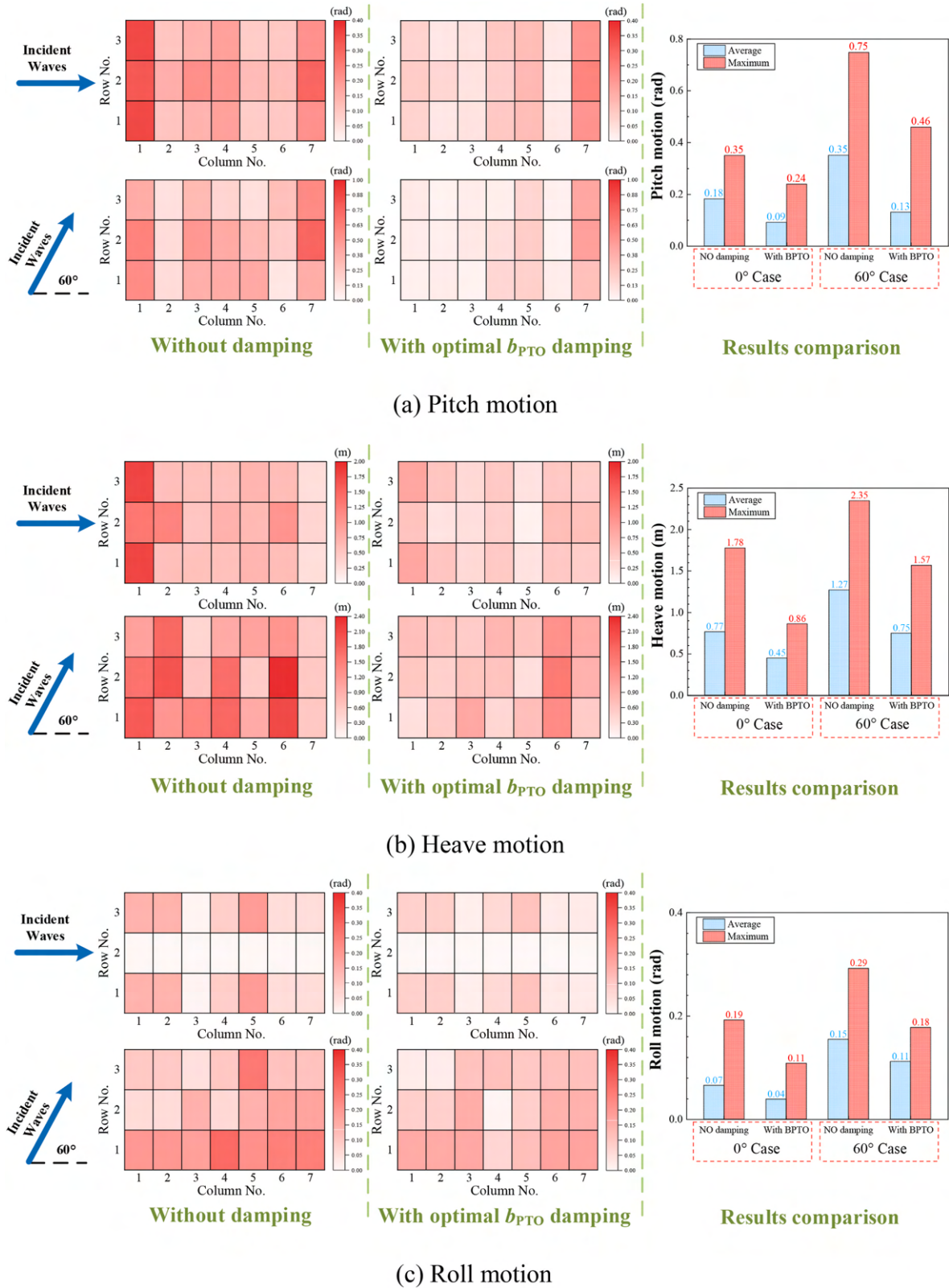
Fig. 18. Impact of optimal b_{PTO} damping on the motion response of the array at T = 5.3 s.
