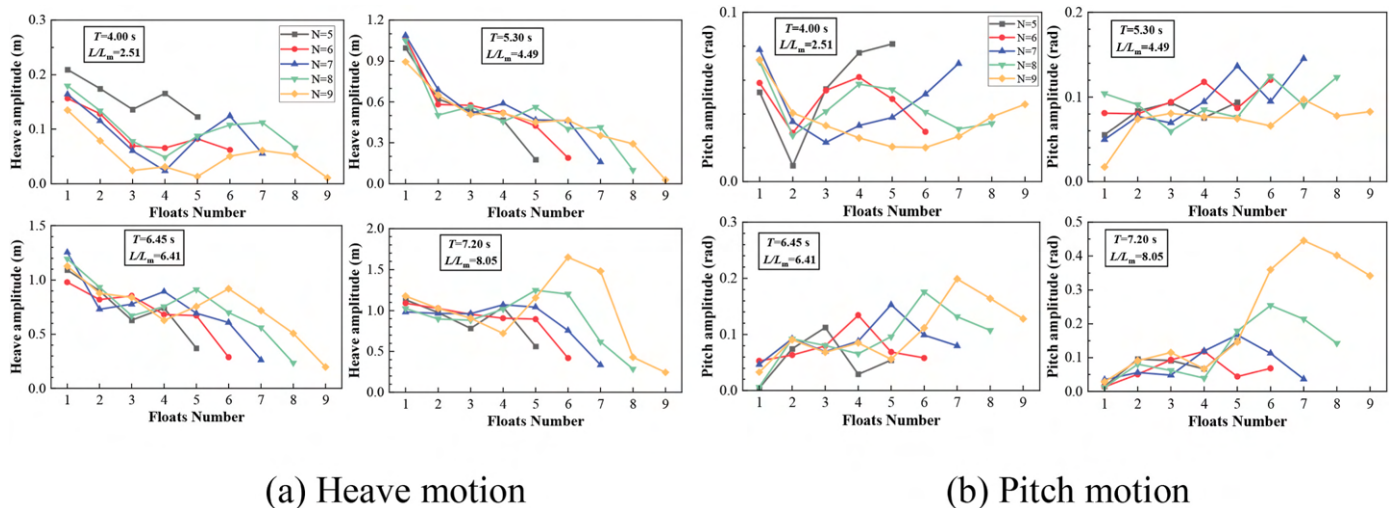
Fig. 11. Motion responses of a single-row array with varying numbers of floats at four representative wave periods ( 0^\circ wave incidence).
