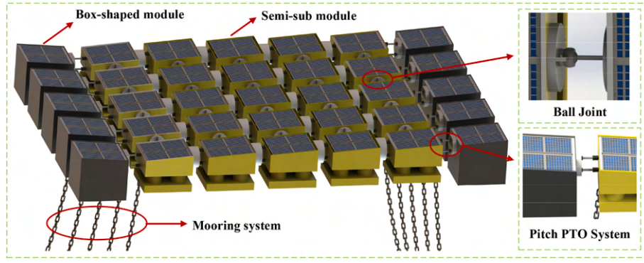
Fig. 1. Design diagram of the novel floating photovoltaic array system.
