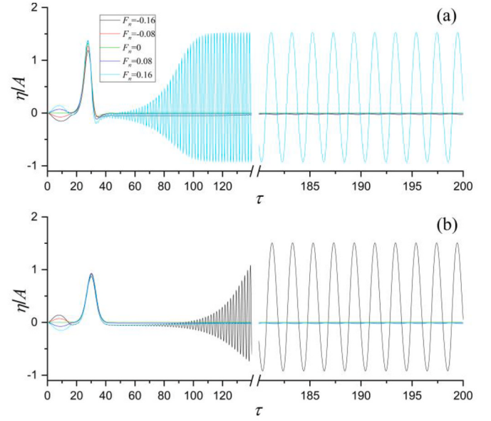
Fig. 11. Histories of waves at A/h = 0.09 ; (a) left side; (b) right side.
