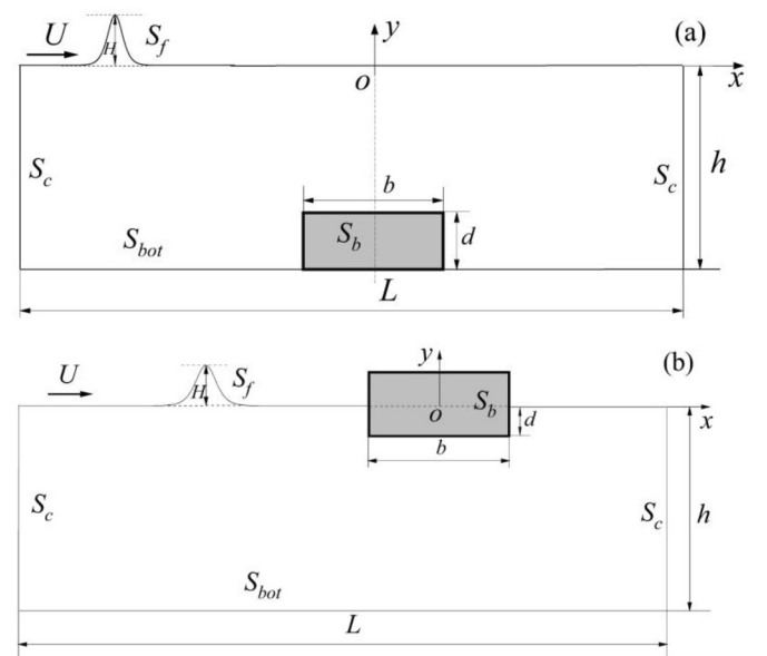
Fig. 1. A sketch of a solitary wave interactions with a body in a current; (a) An underwater and bottom-mounted rectangular cylinder; (b) A rectangular cylinder on free surface.
