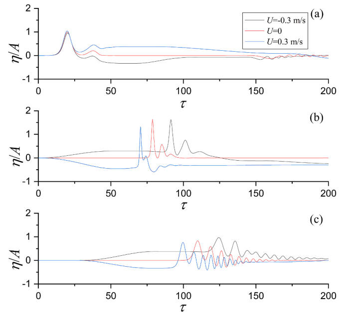
Fig. 4. Wave histories at d/h = 0.6 (a) x/h = -29 ; (b) x/h = 19 ; (c) x/h = 49 .
