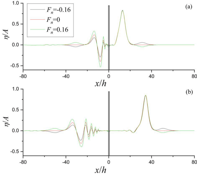
Fig. 15. Wave profiles at (a) \tau = 40 ; (b) \tau = 60 .
