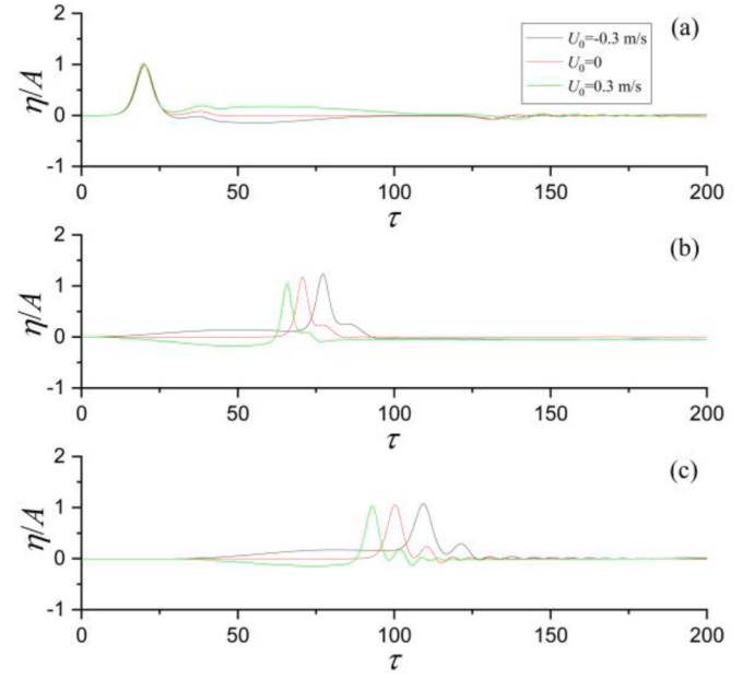
Fig. 8. Wave histories at d/h = 0.3 ; (a) x/h = -29 ; (b) x/h = 19 ; (c) x/h = 49 .
