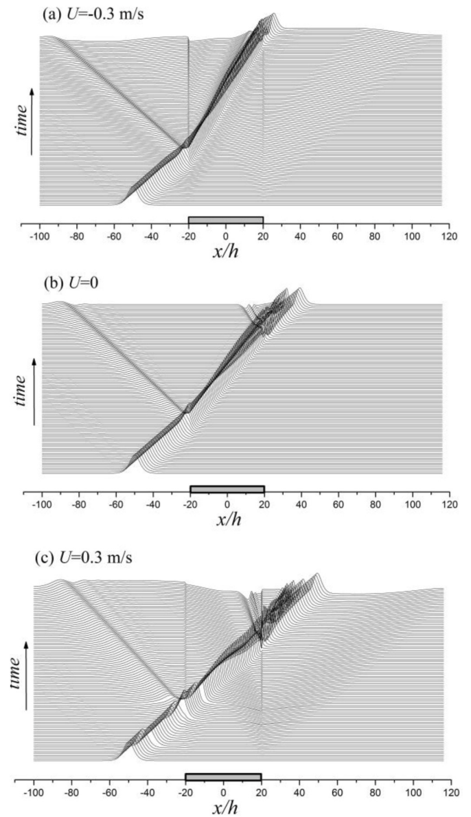
Fig. 5. Snap shots of wave profile from \tau = 0 to 100 with time interval \Delta\tau = 1 and A/h = 0.1 .
