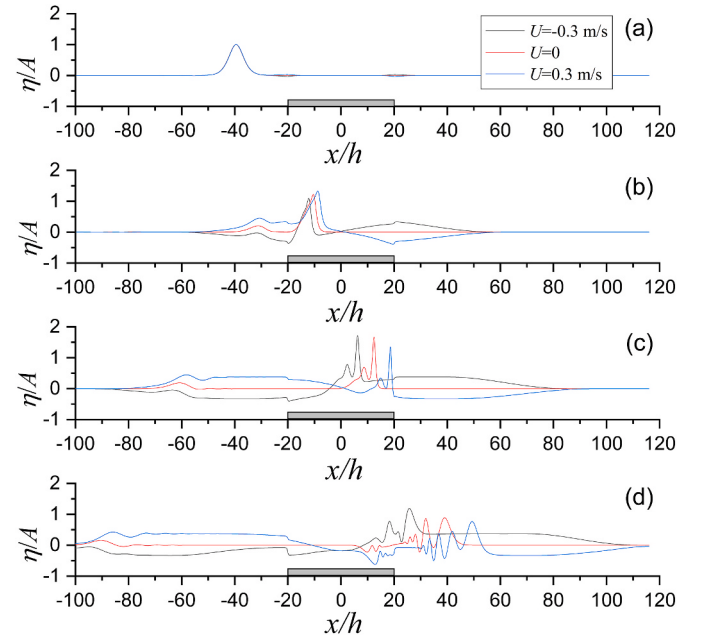
Fig. 3. (a) Wave profiles at (a) \tau = 10 ; (b) \tau = 40 ; (c) \tau = 70 (d) \tau = 100 at A/h = 0.1 .
