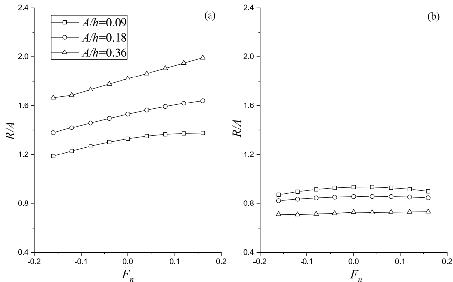
Fig. 16. Wave run-ups versus the Froude number; (a) left side; (b) right side.
