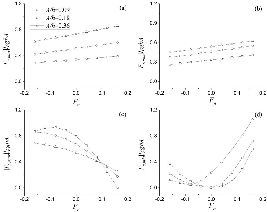
Fig. 17. Force peak and trough versus Froude number.
