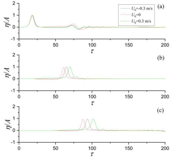
Fig. 9. Wave histories at d/h = 0.6 and b/h = 2 ; (a) x/h = -29 ; (b) x/h = 19 ; (c) x/h = 49 .
