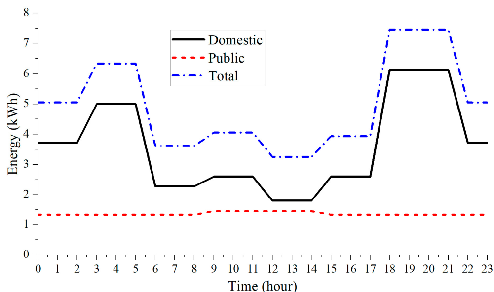
Figure 5. The hourly electricity demand of Sub-village Kalenan.
