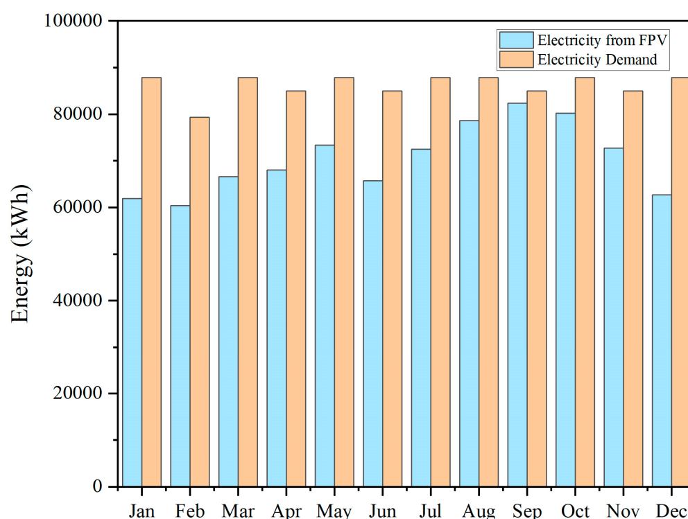
Figure 9. Energy simulation results for Bungin Island.
