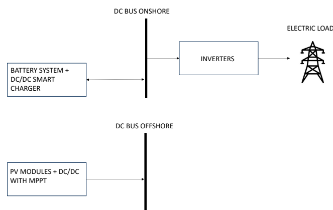
Figure 6. Sketch of the floating PV plants.
