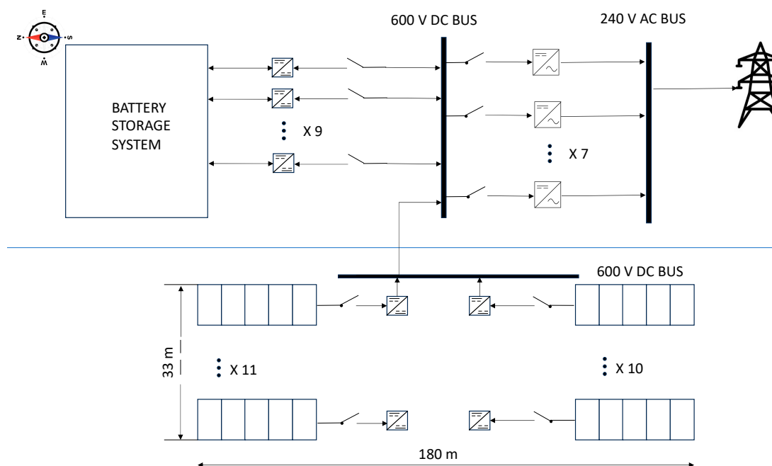
Figure 15. Bungin electrical drawing.
